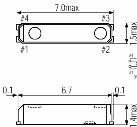
Figure 1) Top, Side and End View
