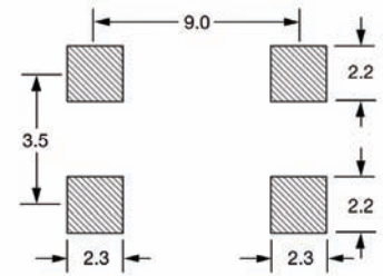
Figure 3) Land Pattern
